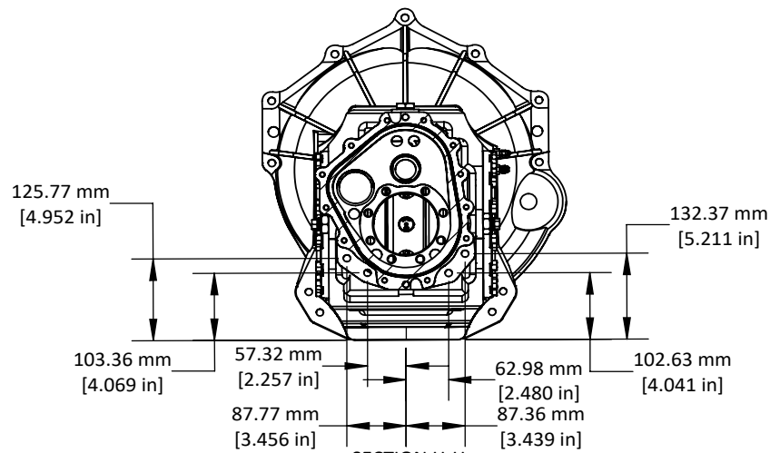
SECTION H-H Main Case Mounting Hole Detail
