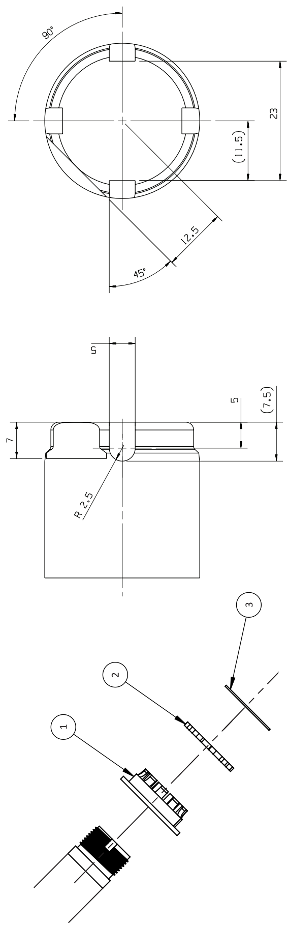
Notches and flat must be added to end of pinion shaft, as shown. Dimensions in millimeters.
